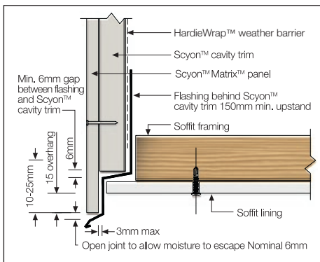
FIGURE 33 FACADE/SOFFT JUNCTION
