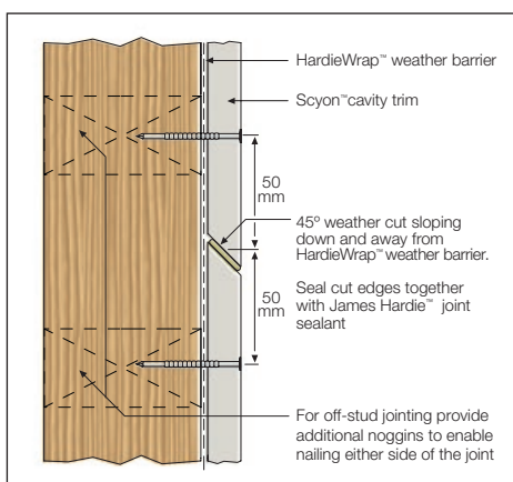
FIGURE 10 SCYON™ CAVITY TRIM BUTT DETAIL
